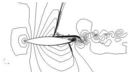
Fig. 1 Velocity contours from the DES solution.
