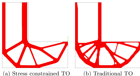
Figure 1: Designs for an L-shaped beam in 2D
