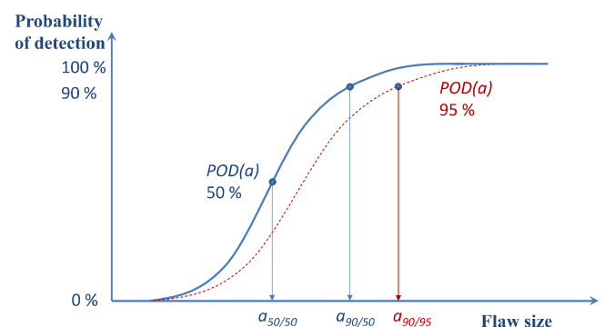
Fig. 1 POD curve with 95 % lower confidence limit.
