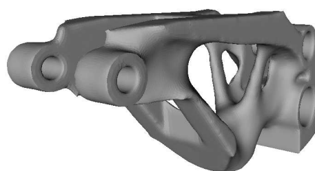
Figure: ALM load introduction bracket
