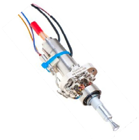
ECAPS 1N HPGP Thruster
