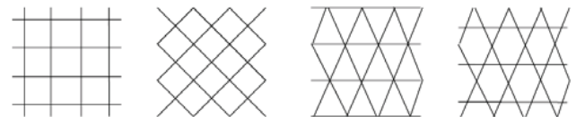
Fig. 1 From left to right: Orthogrid, Anglegrid, Isogrid and Anisogrid
