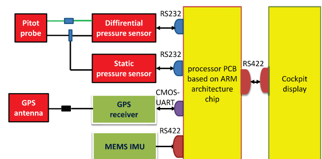
Fig.1 system hardware architecture
