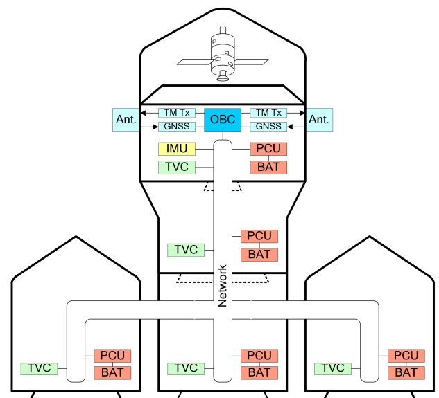
Fig. 1 Tentative launcher avionics configuration
