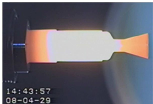
Hot-firing of a 1N HPGP Thruster
