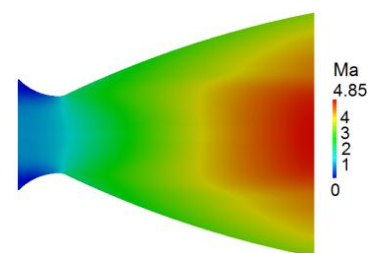
Figure 1. Mach number inside the nozzle.
