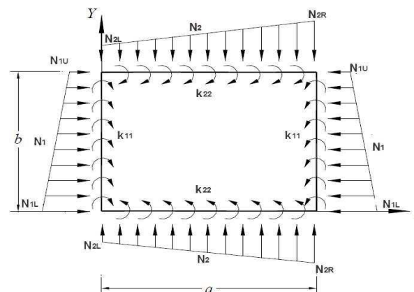
Figure 1: Model of Rotationally Restrained Plate
