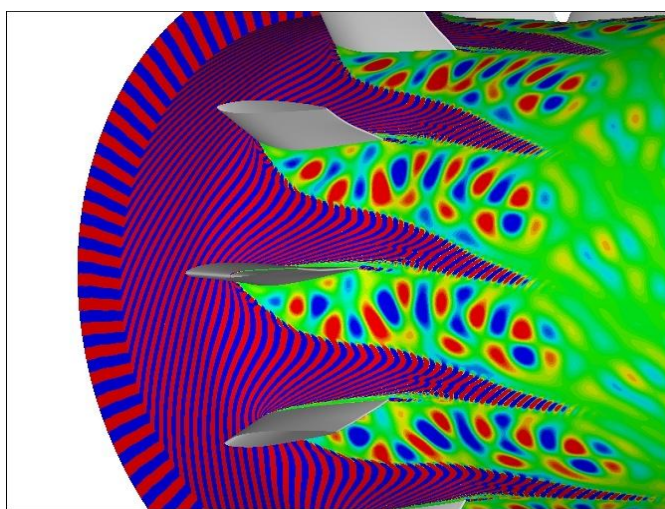
Separated turbine outlet guide vane
