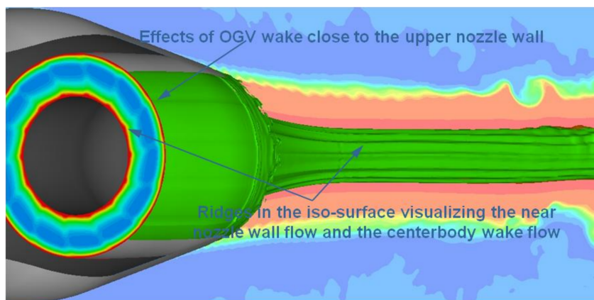
Co-Axial jet noise prediction
